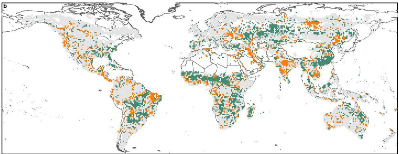
Nighttime Active Fire Detections
