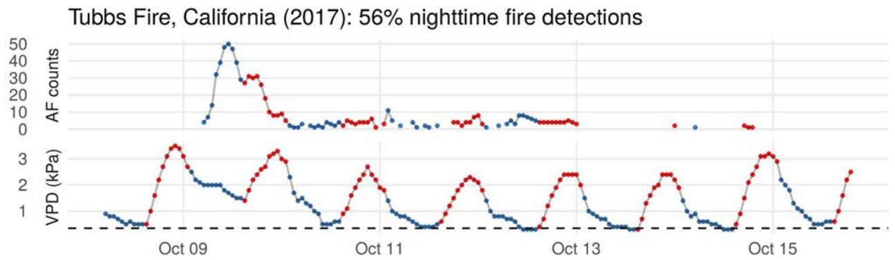
Extended Data Fig. 3 | Diurnal oscillations of weather and active fire counts, displaying hourly time series of GOES active fire detections 19 and ERA-5 38 VPD for two fire events in the United States. A dashed line marks the
