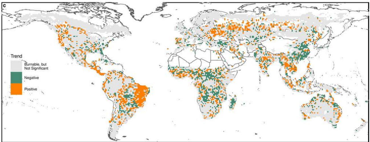
Percent Nighttime Active Fire Detections
