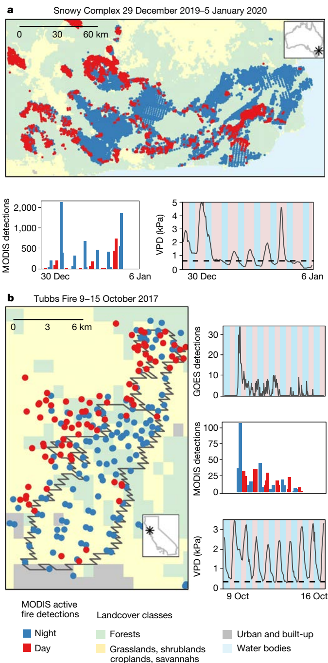
Fig. 3 | Two wildfires illustrate the relationship between night-time VPD and fire activity. a, b. Night-time fires spread rapidly during the Snowy Complex wildfire in southeast Australia ( a ), and the Tubbs wildfire in California ( b ) when VPD_{min} > VPD_e . Night-time MODIS active fire detections 20 represented 76% and 56% of total detections by event, respectively. Time series of the VPD 38 oscillation from day to night are shown, with blue (pink) shading in the background indicating night (day), as well as the number of active fire detections from MODIS (for both wildfires, n = 8,163 and n = 212 , respectively) and GOES 19 (for the Tubbs wildfire only). The dashed lines are the landcover-specific VPD thresholds for temperate evergreen broadleaf forests (0.6 kPa) and temperate woody savannahs (1 kPa), which were the predominant landcover classes for the Snowy Complex and Tubbs fire, respectively. In the first few days of each wildfire, VPD_{min} (troughs in the insets) was well above the VPD threshold. Figure developed using R software.
