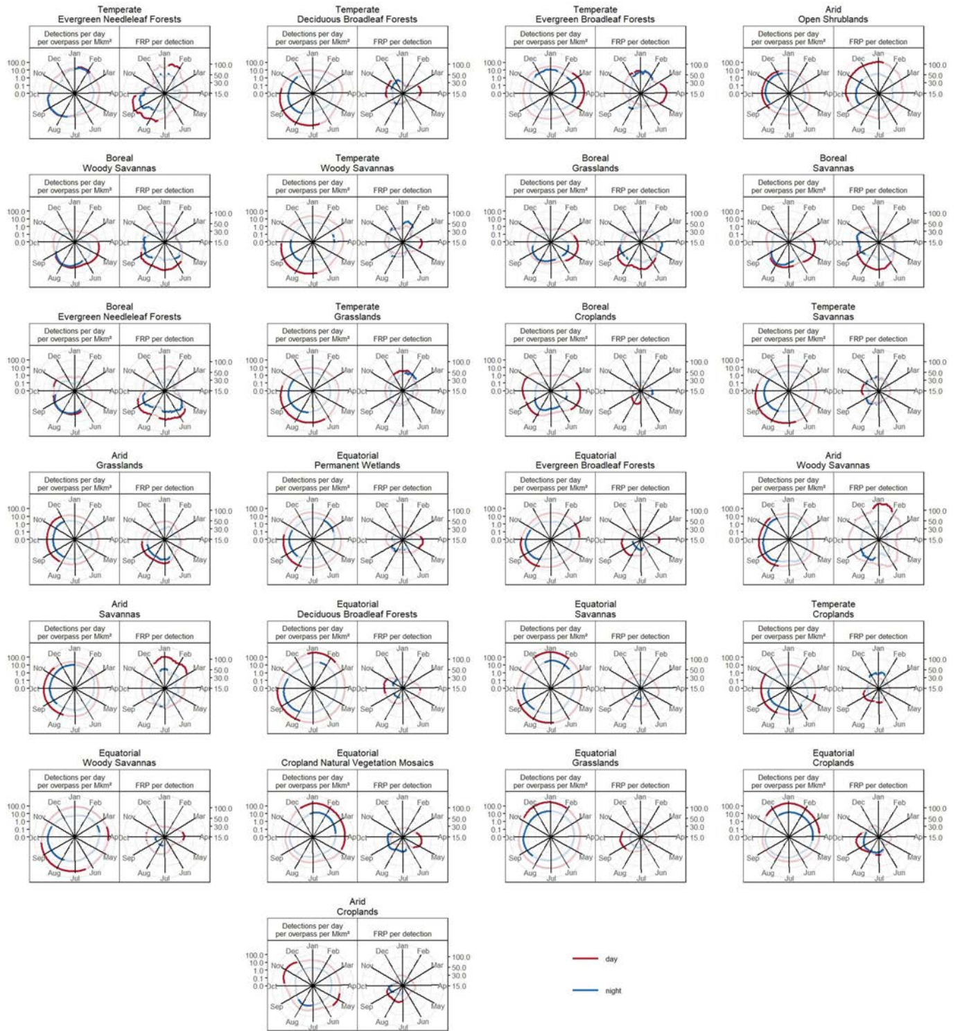
Extended Data Fig. 2 | Observed peak fire season (dark lines) based on MODIS active fire detections (MCD14ML) 20 . Each line, smoothed using a 31-day window, represents the expected number of day or night active fire detections per overpass per million km 2 (left facets) or the expected day or night FRP per detection (right facets) for each landcover type averaged across
