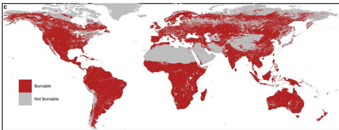
Extended Data Fig. 1 | Climate and landcover classifications used in VPD threshold analysis shown at 1° grid cell resolution. a, The Köppen–Geiger climate classifications 69 . b, The MODIS MOD12Q1 landcover 68 . c, Areas in red fill
