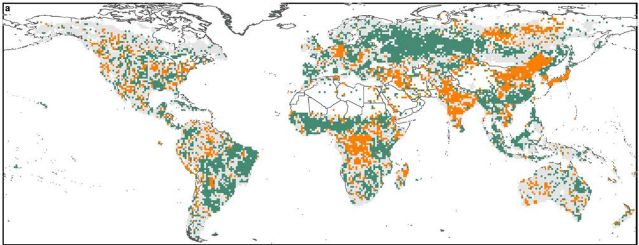
Daytime Active Fire Detections
