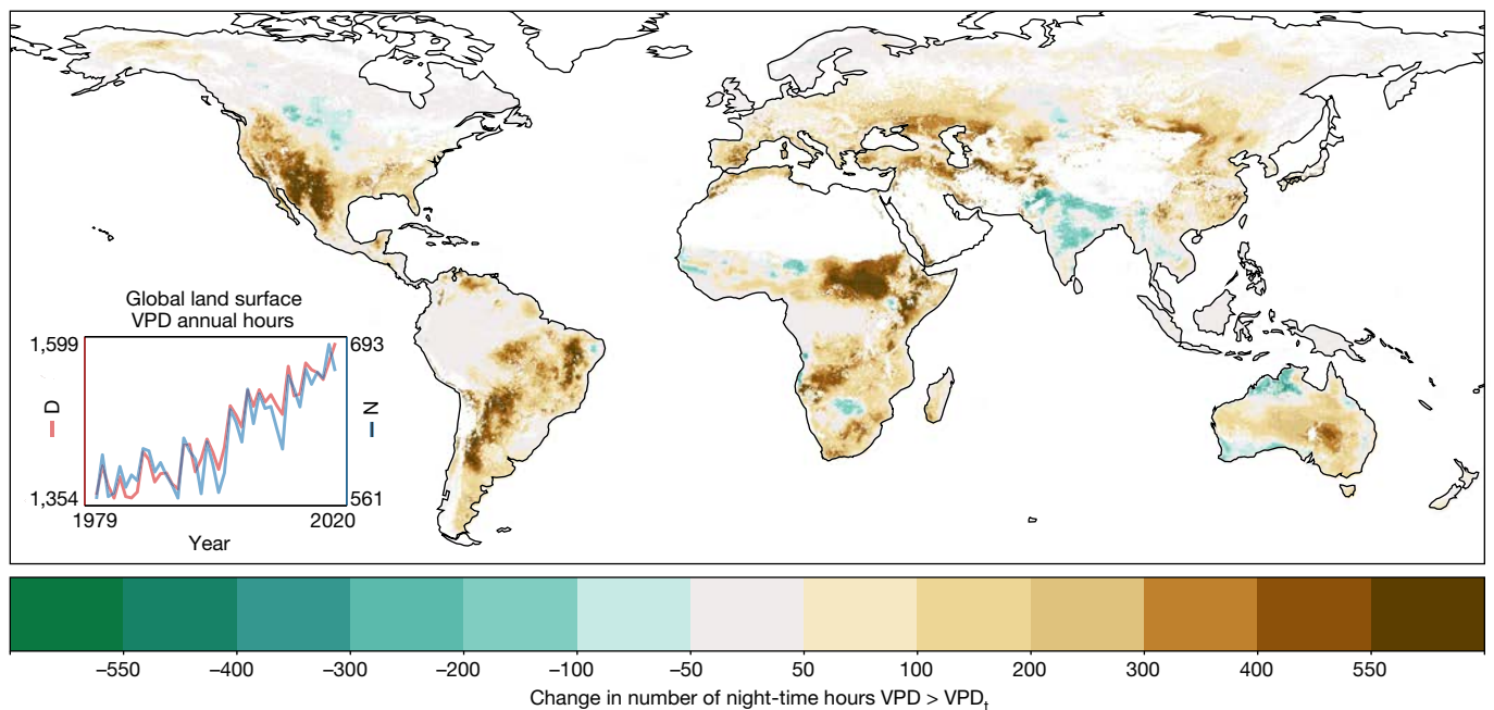
Fig. 4 | The annual number of flammable night-time hours when VPD > VPD_t increased by over a third from 1979 to 2020. Forty-seven per cent of burnable lands (by pixel) had significant ( P < 0.05 ) positive trends in the number of night-time hours above the VPD^{38} threshold (80% had increases in total),
